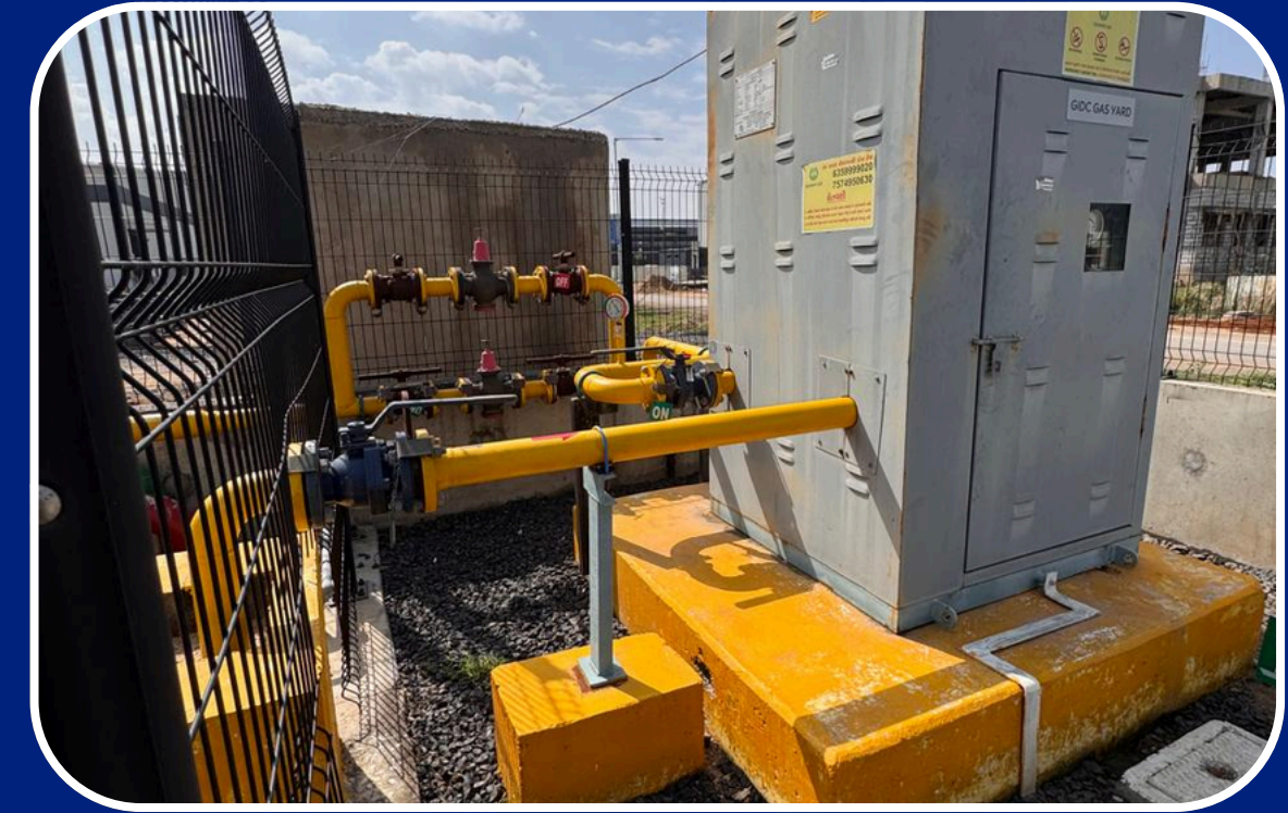
PNG Gas System
